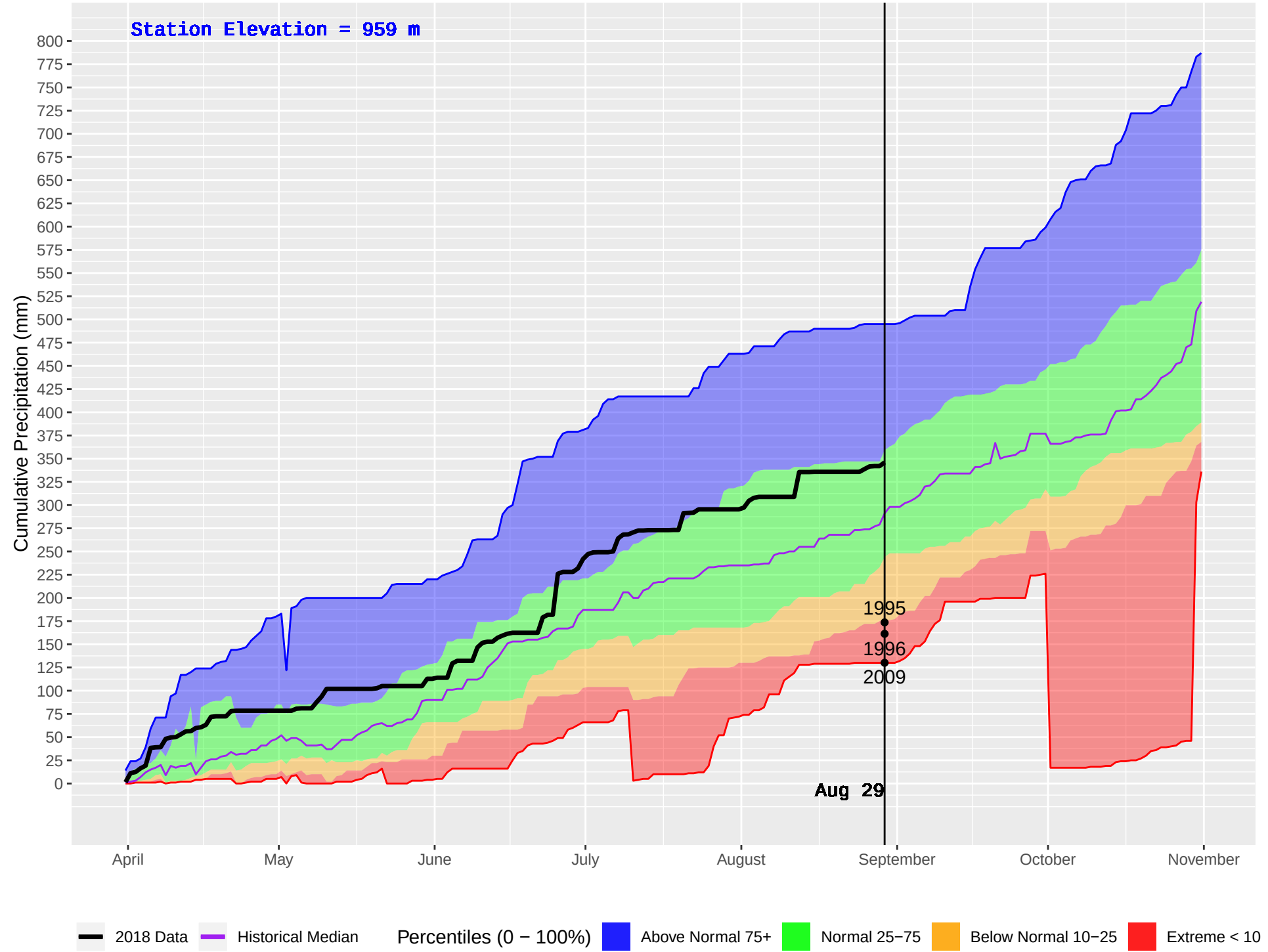
WELLS GRAY (266) : Historical (1994–2016) and Current (2018) Daily Cumulative Precipitation
