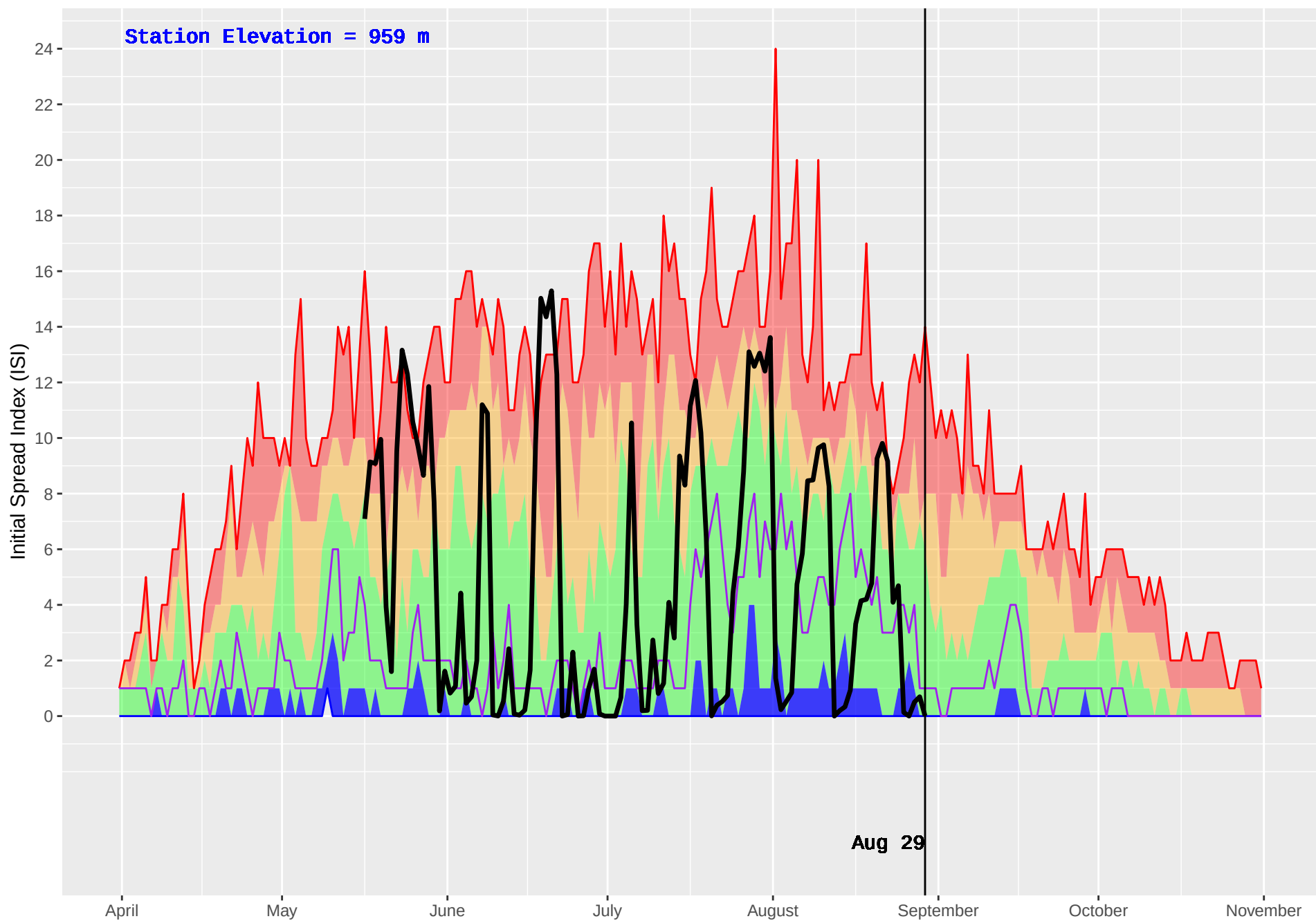
WELLS GRAY (266) : Historical (1994–2016) and Current (2018) Daily Initial Spread Index (ISI)
