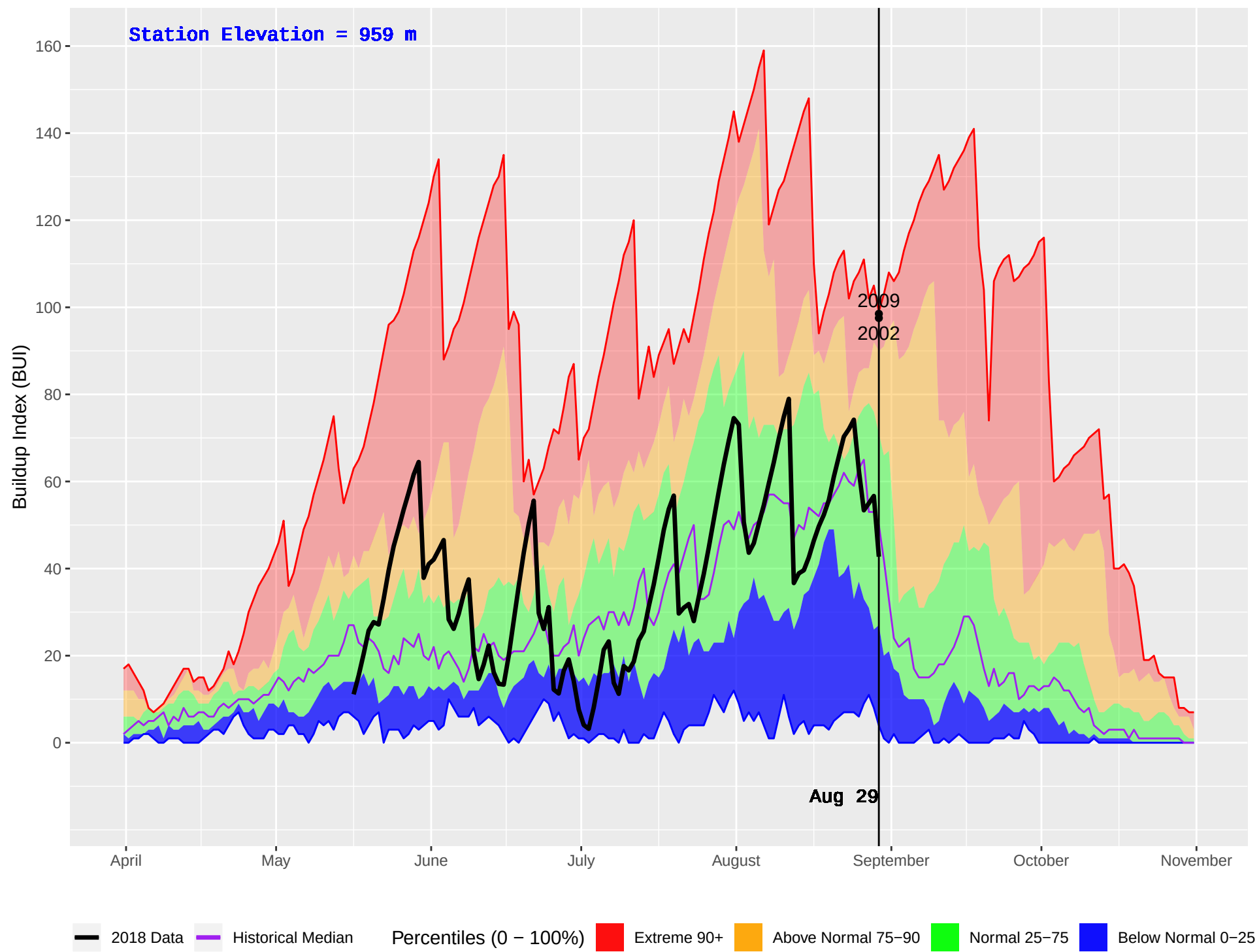
WELLS GRAY (266) : Historical (1994–2016) and Current (2018) Daily Buildup Index (BUI)
