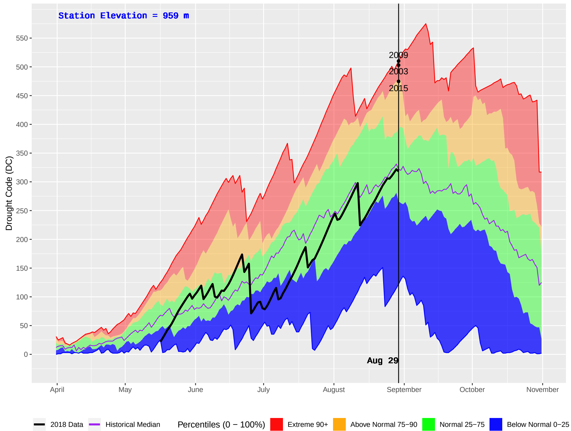
WELLS GRAY (266) : Historical (1994–2016) and Current (2018) Daily Drought Code (DC)
