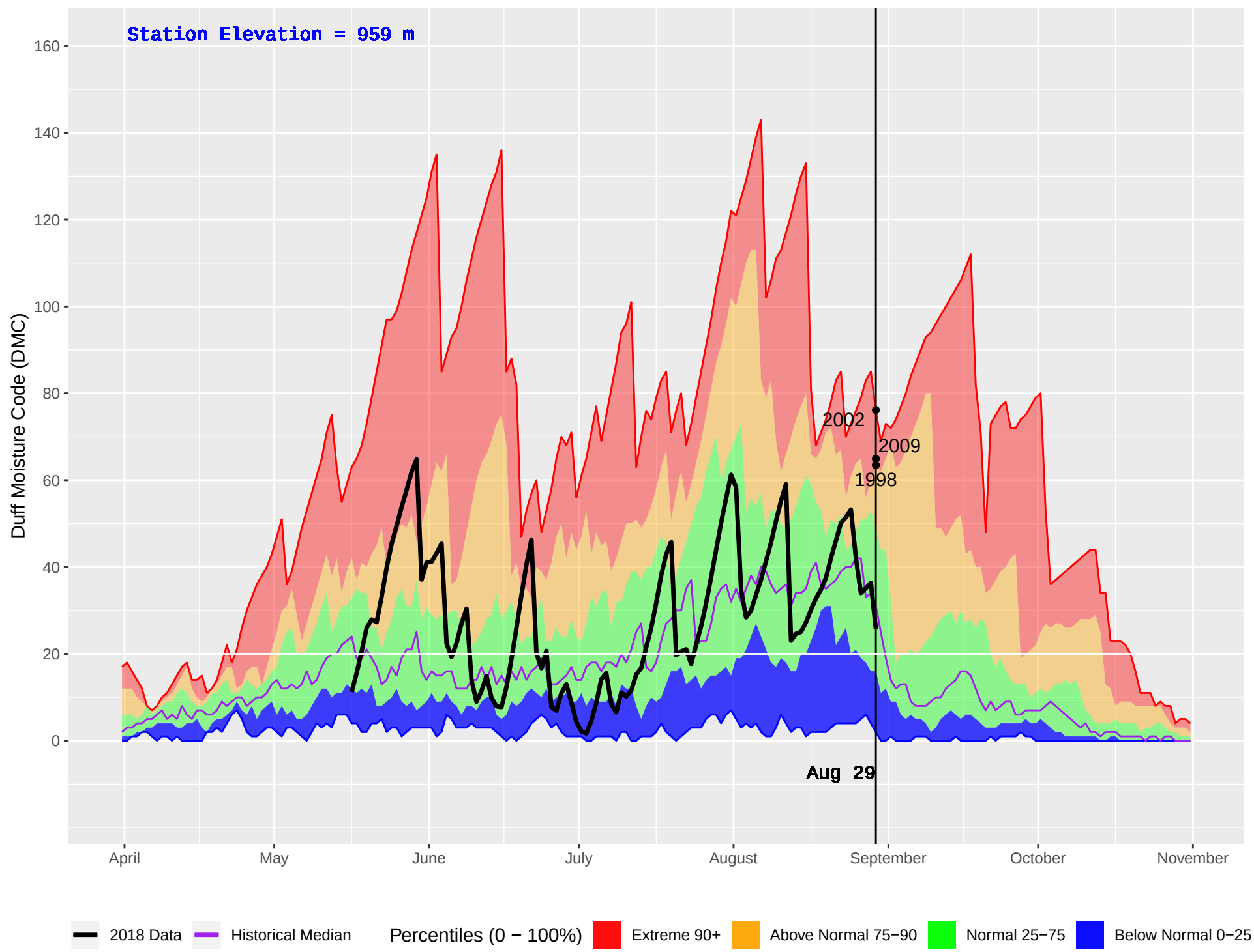
WELLS GRAY (266) : Historical (1994–2016) and Current (2018) Daily Duff Moisture Code (DMC)
