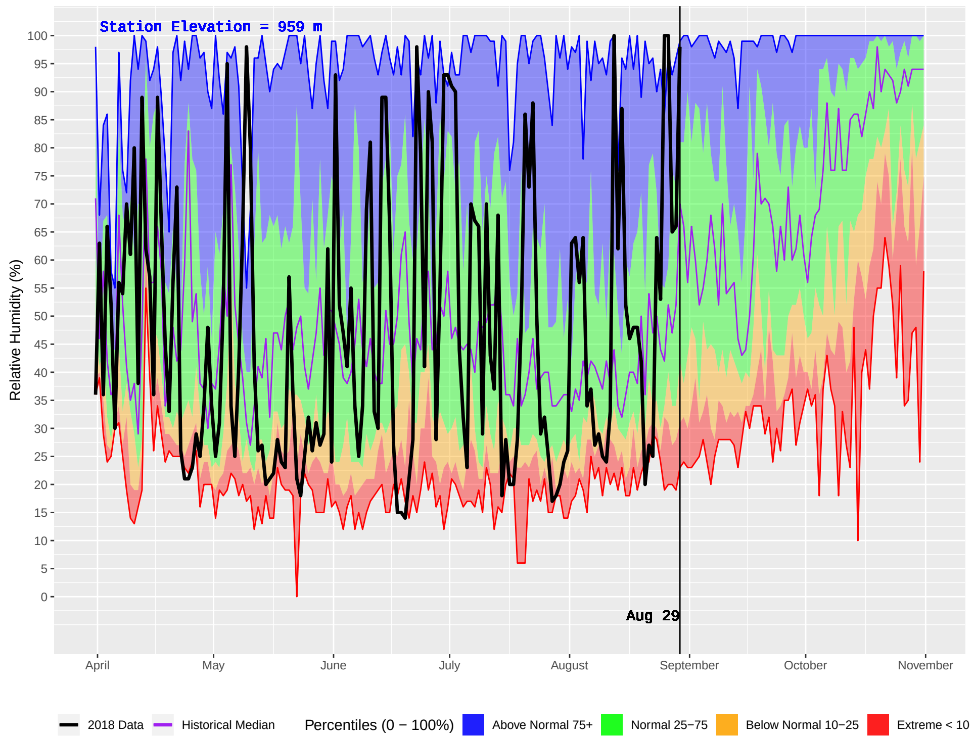
WELLS GRAY (266) : Historical (1994–2016) and Current (2018) Daily Relative Humidity
