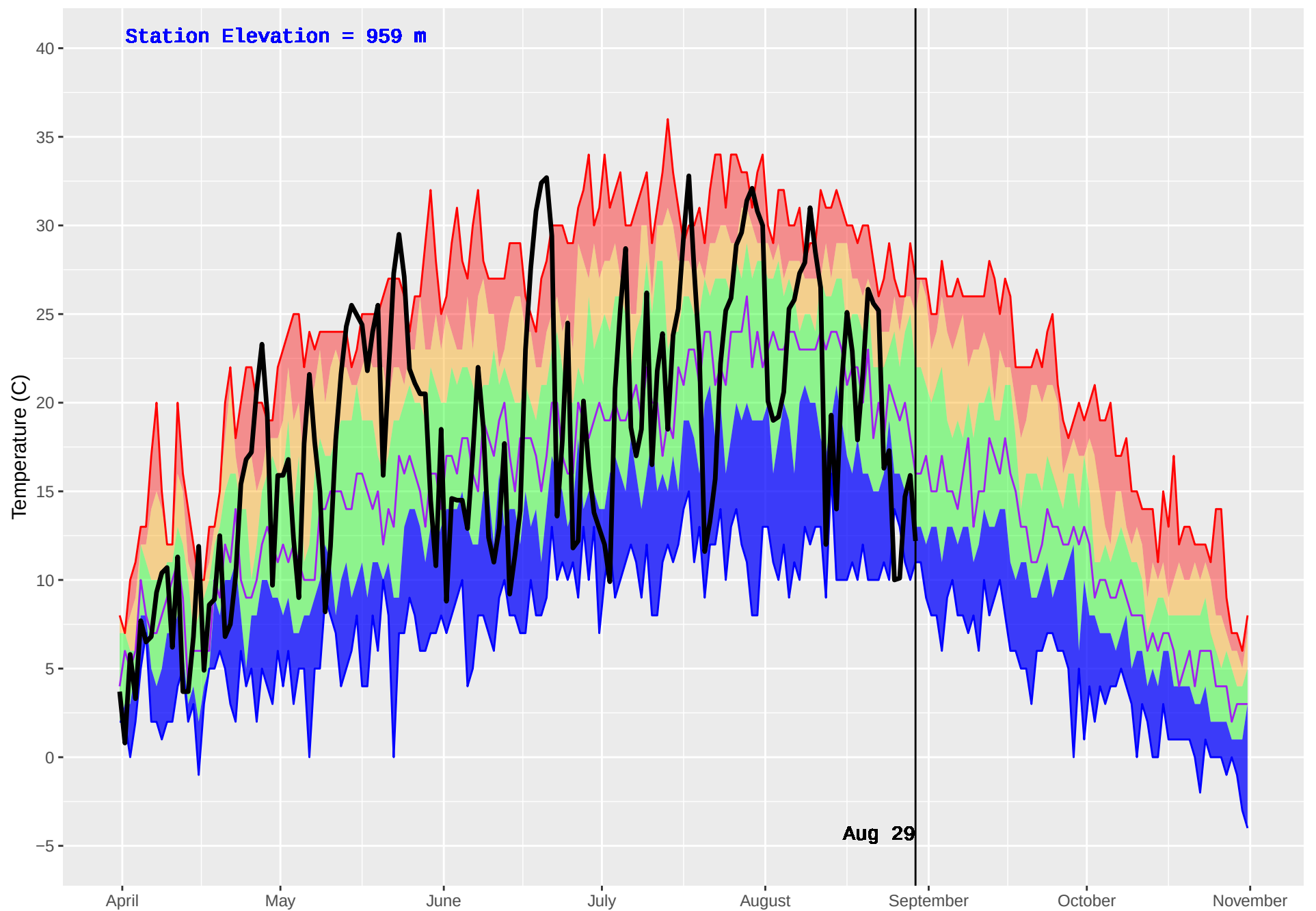
WELLS GRAY (266) : Historical (1994–2016) and Current (2018) Daily Temperature
