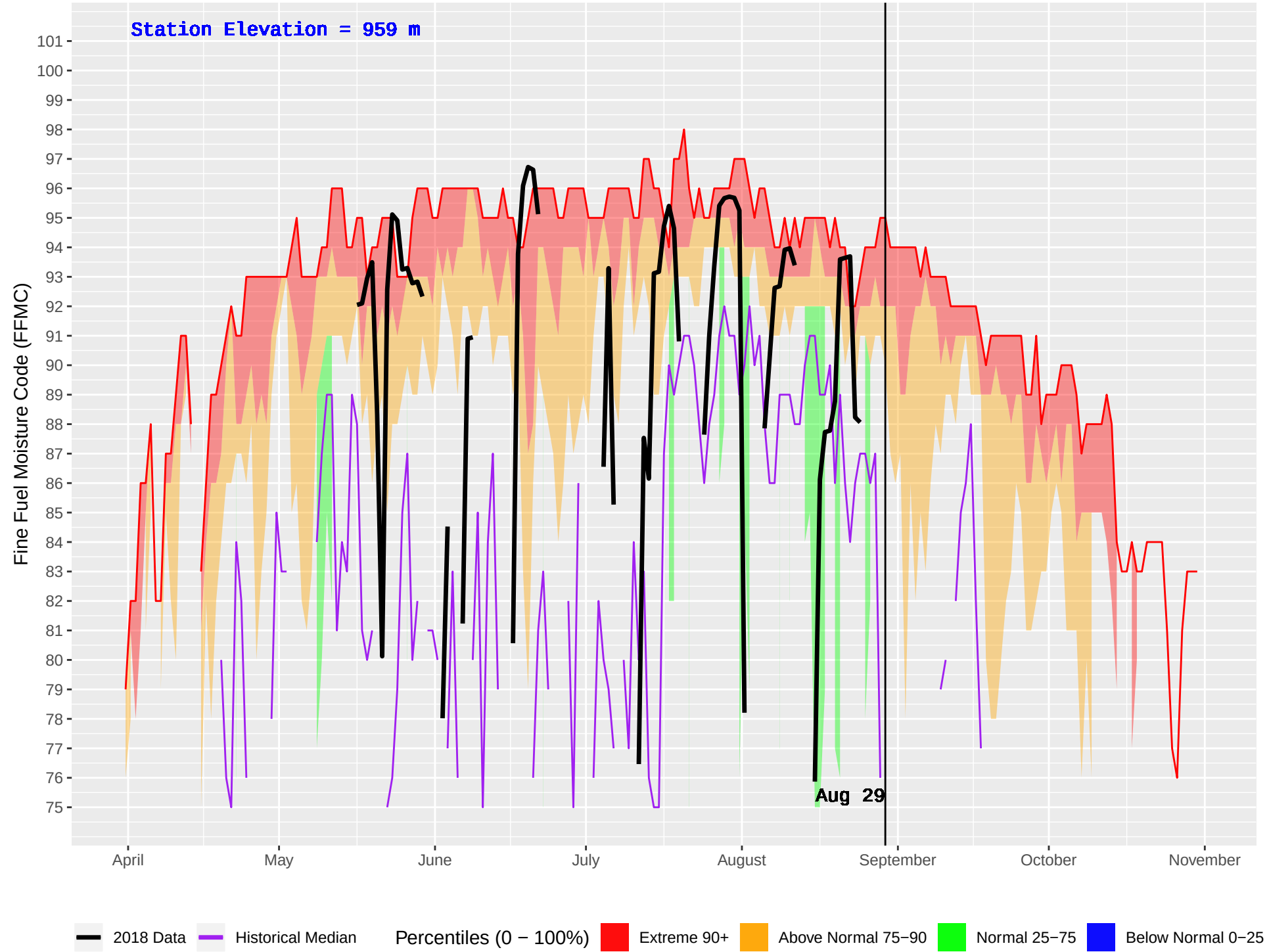
WELLS GRAY (266) : Historical (1994–2016) and Current (2018) Daily Fine Fuel Moisture Code (FFMC)
